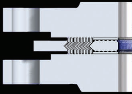
Flange with WRI-LP Corrosion Protection
