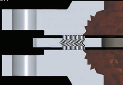
Flange with WRI-LP Corrosion Protection
