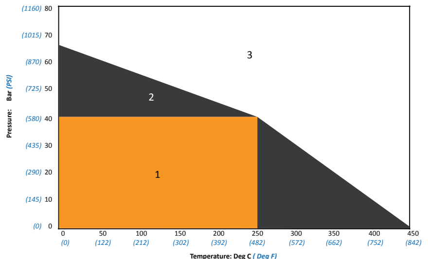
L460 PRESSURE / TEMPERATURE GRAPH
